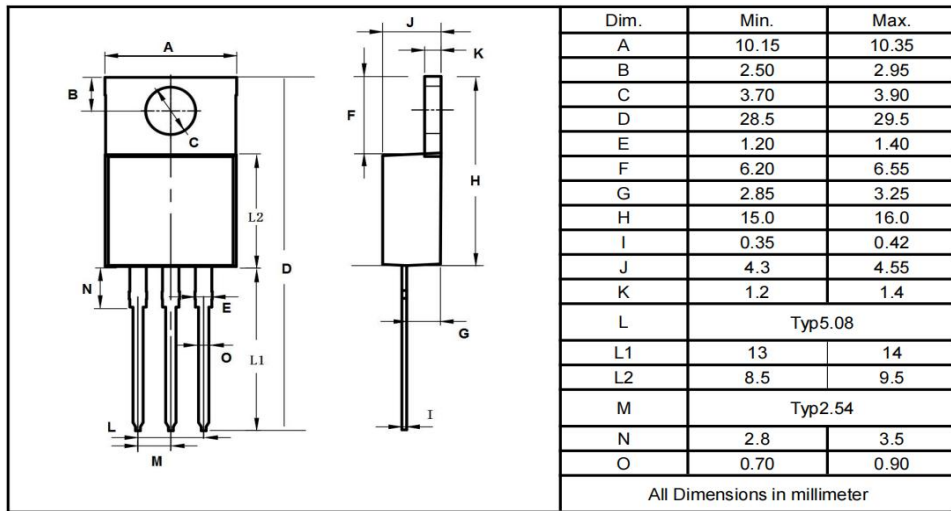
TO-220F
